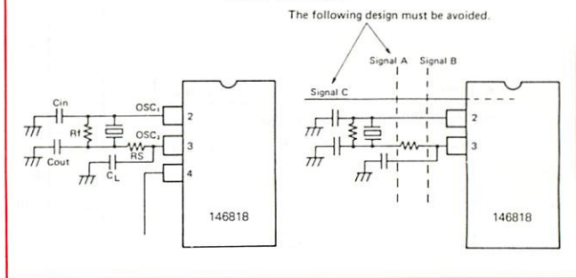
Figure 11 Note for Board Design of the Oscillation Circuit
