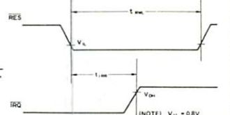
Figure 5 IRQ Release Delay (from RES)
