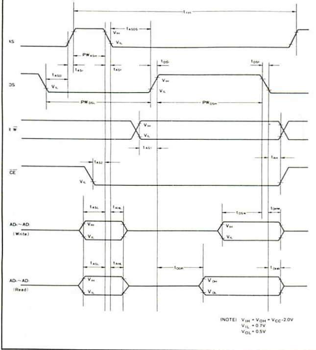
Figure 1 Bus read, write timing (6800 family)
