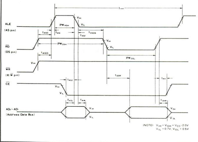
Figure 2 Read timing (8085 family)
