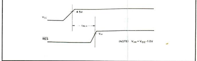
Figure 7 RES Release Delay
