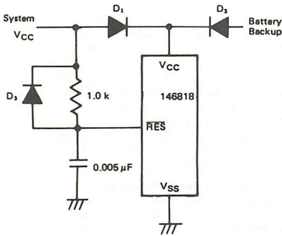
Figure 16 Typical Powerup Delay Circuit for RES
