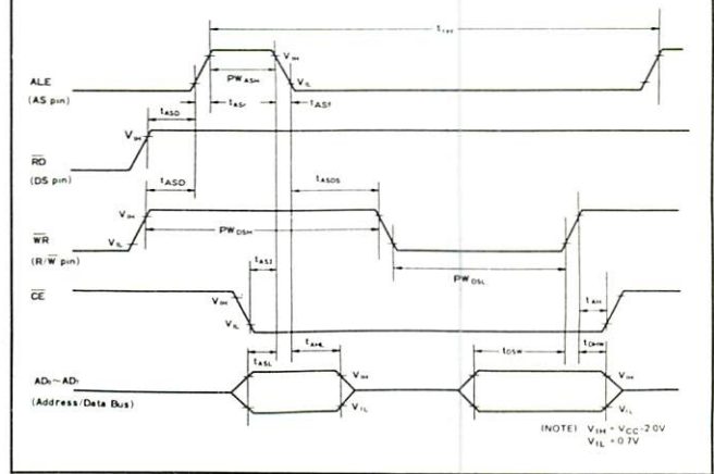
Figure 3 Write timing (8085 family)
