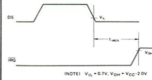
Figure 4 IRQ Release Delay (from DS)
