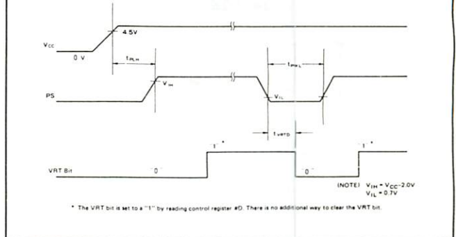
Figure 6 VRT Bit Clear Timing
