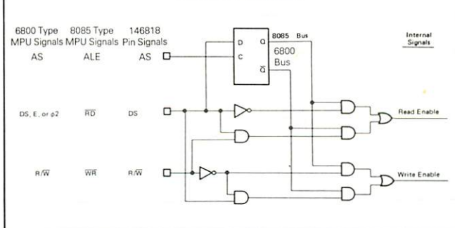
Figure 12 Functional Diagram of the Bus Control Circuit
